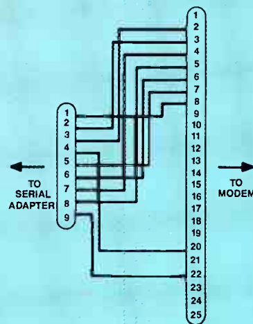
Typical IBM-AT computer-to-modem interface cable.
