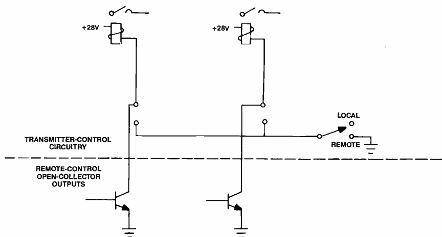
Figure 9. Be wary of open-collector outputs that may bypass the local/remot switch. This creates a safety hazard.
