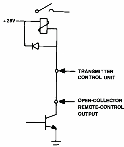
Figure 6. Open-collector control output switches to ground, turning on the relay.
