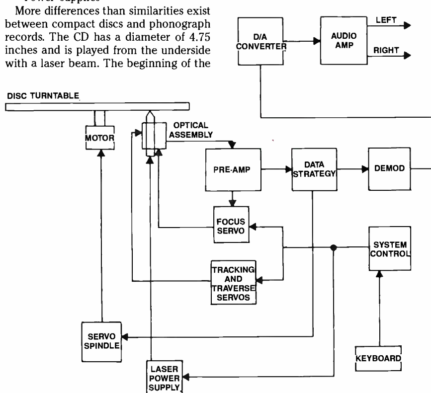
Figure 1. Block diagram of a typical CD player.
