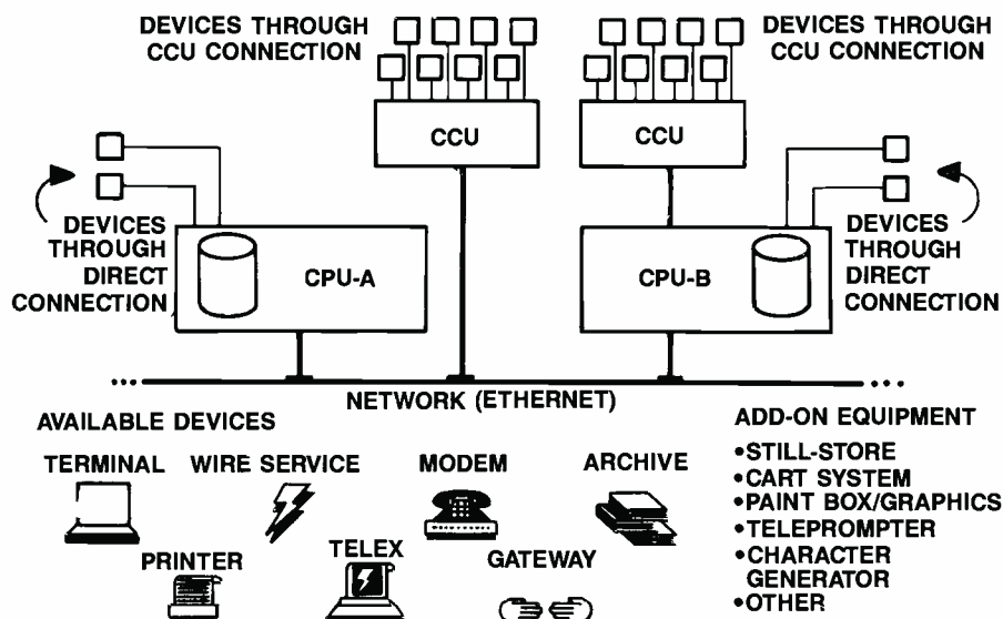
Figure 4. A typical newsroom computer system requires that hardware be installed in many areas of the station.
